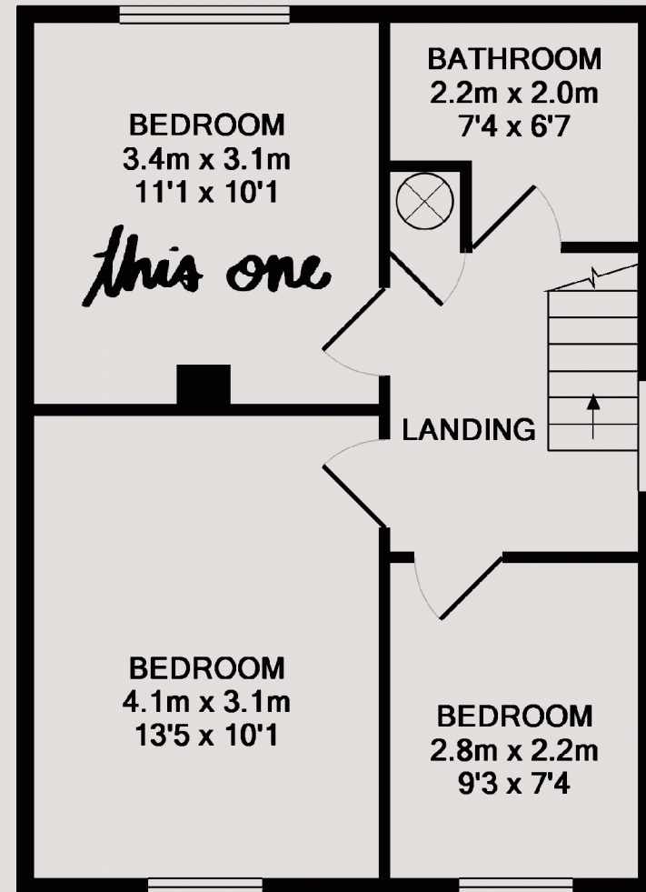
1ST FLOOR
